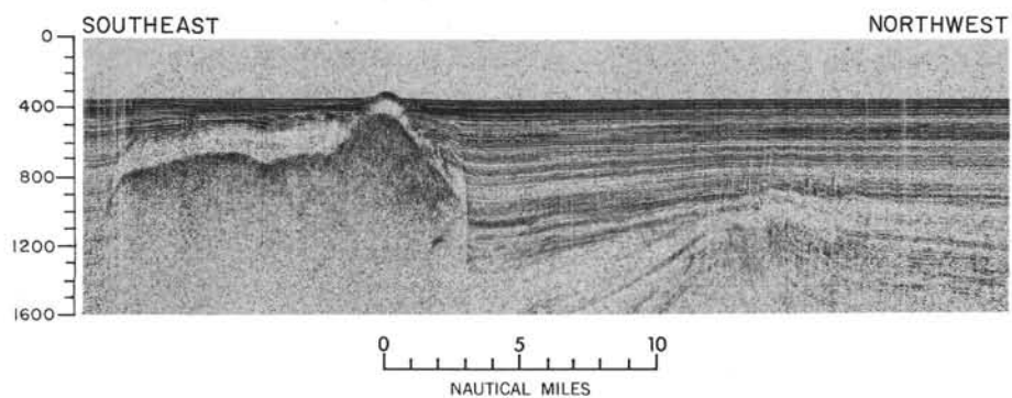
PROFILE OF SIGSBEE ABYSSAL PLAIN AND SIGSBEE KNOLLS AND DOMES
