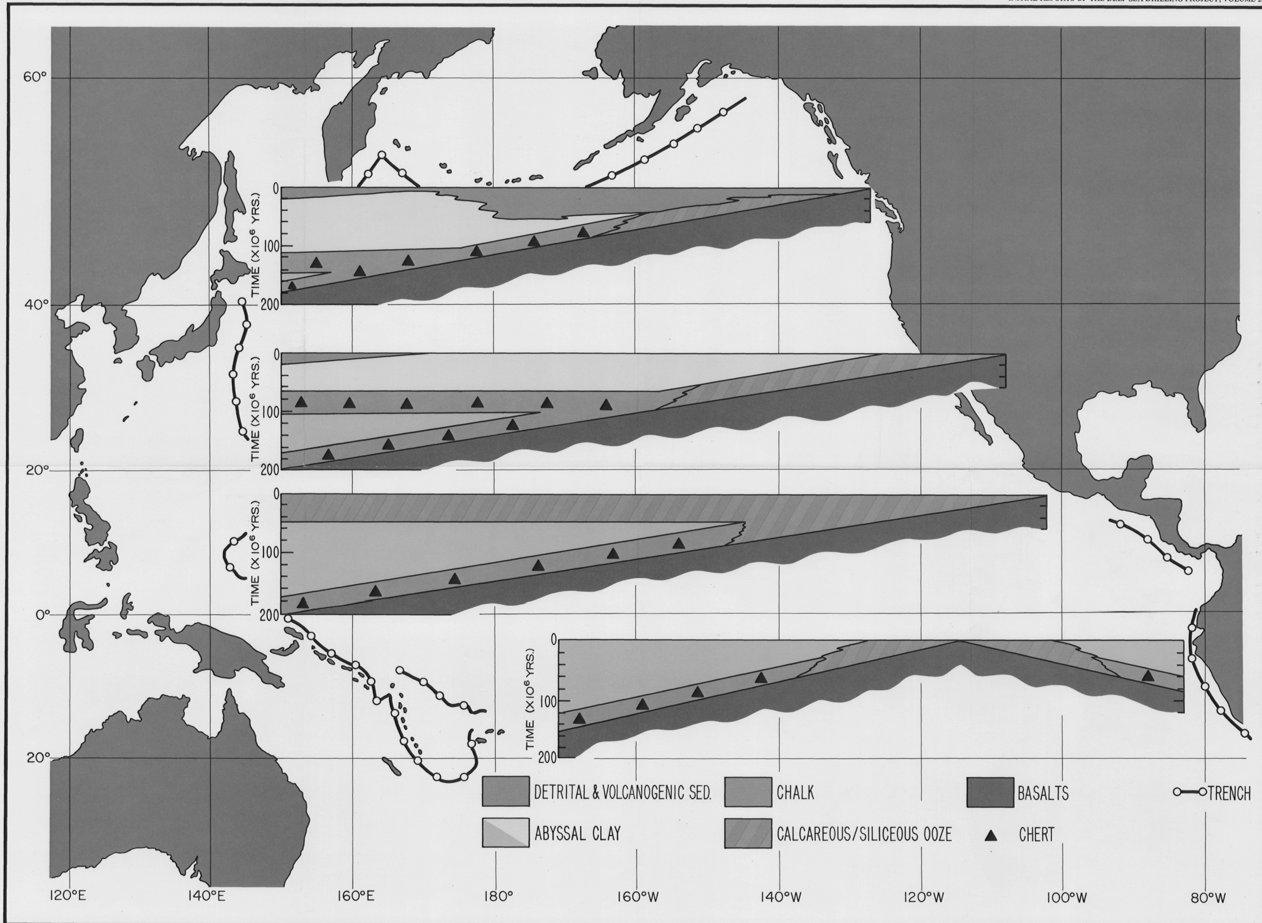
PLATE 2. Computed theoretical distribution of sedimentary facies in the Pacific Ocean according to the analytical model of Pacific sedimentation (see text).
