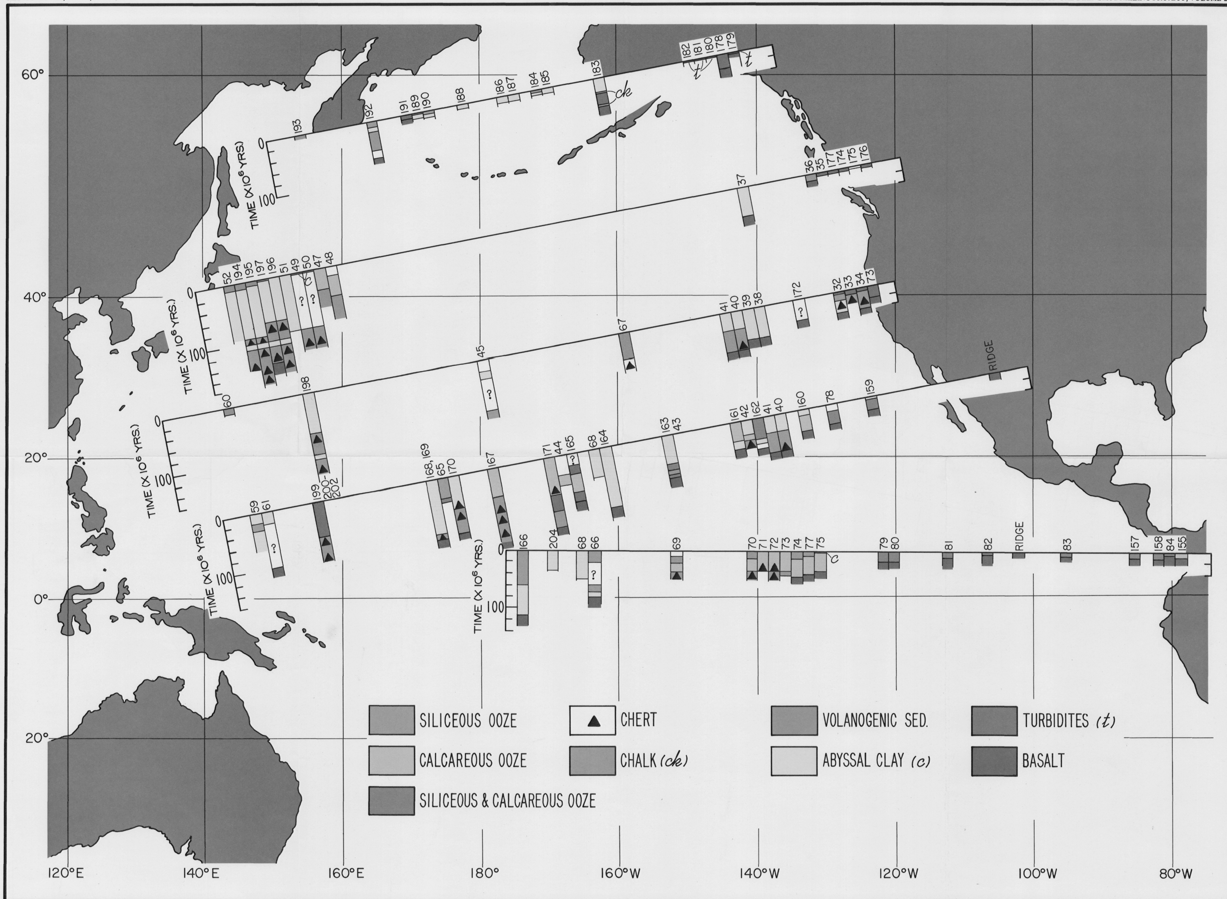
PLATE 3. Summary of lithology vs. age for Pacific DSDP sites through Leg 20. Sites are projected to construct five trans-Pacific profiles.
