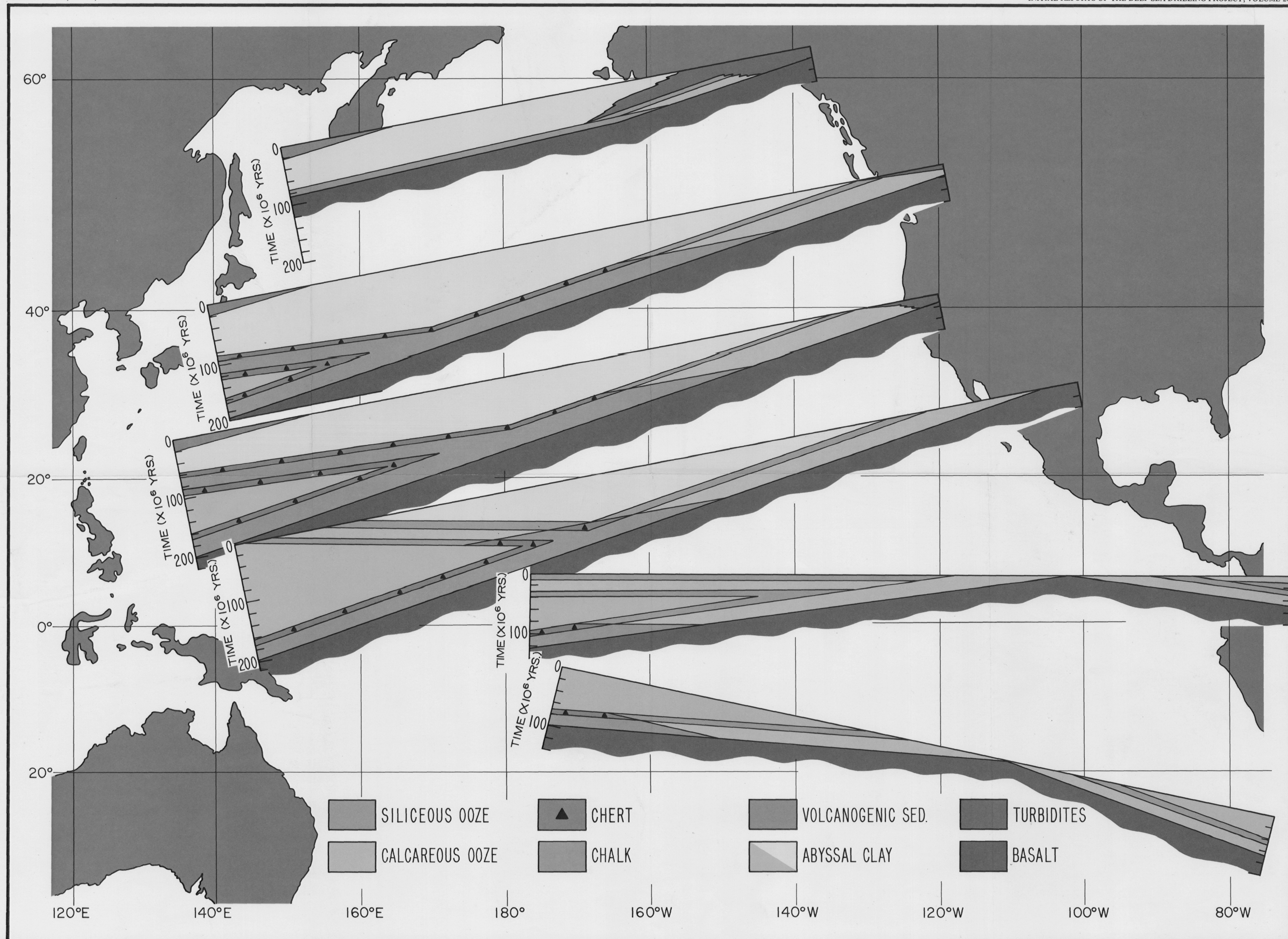
PLATE 4. Lithology vs. age cross sections of the Pacific based on DSDP data through Leg 20.
