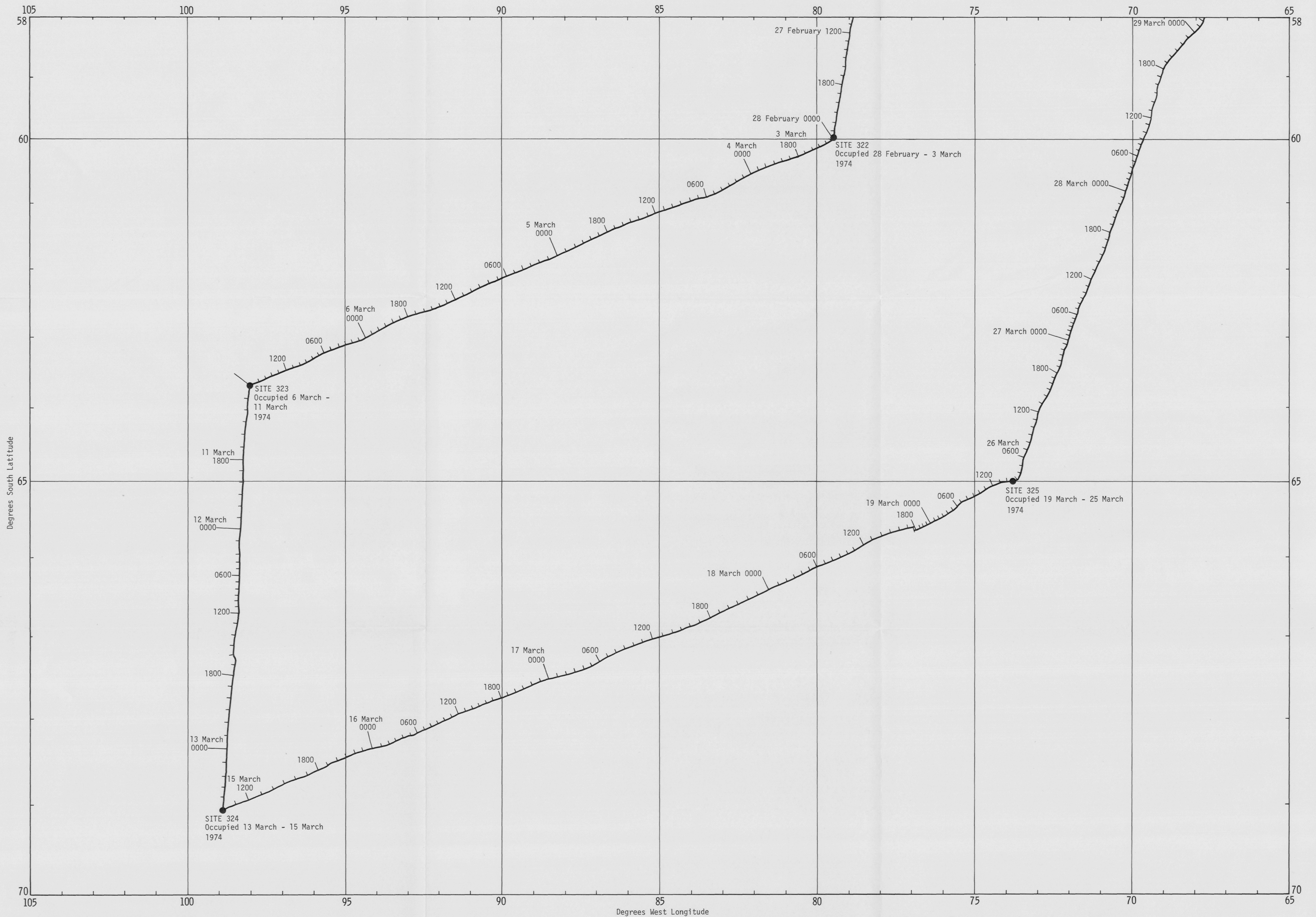
Foldout C - Bathymetric map of the Bellingshausen Basin.
