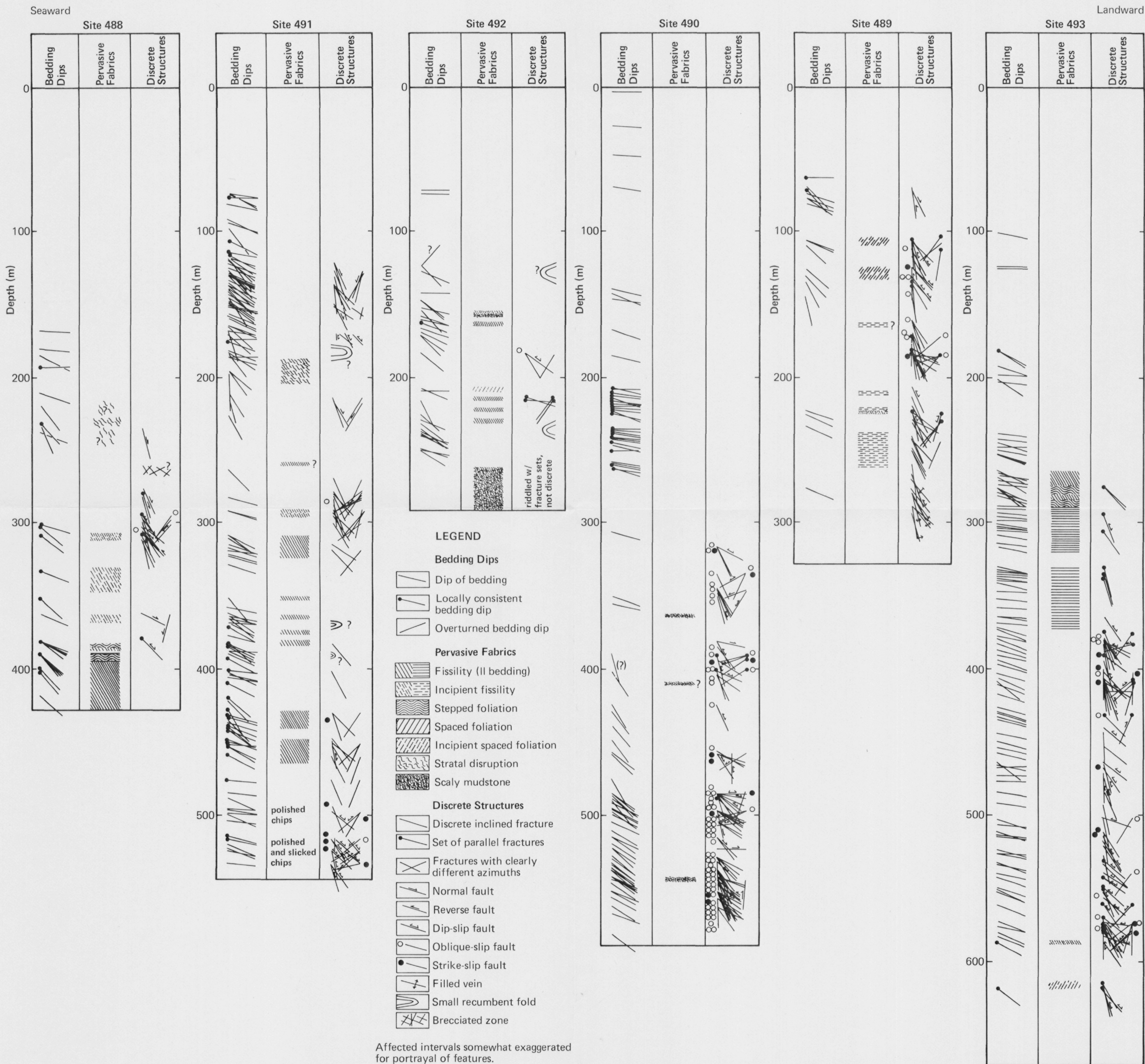
Volume 66: Chapter 40: Figure 3. Graphic structural log depicting location, frequency, and orientation of bedding tilts, penetrative fabrics, and discrete structures for inner trench slope sites, Leg 66. (The sites are arranged geographically, from seaward at the left to landward on the right.)
