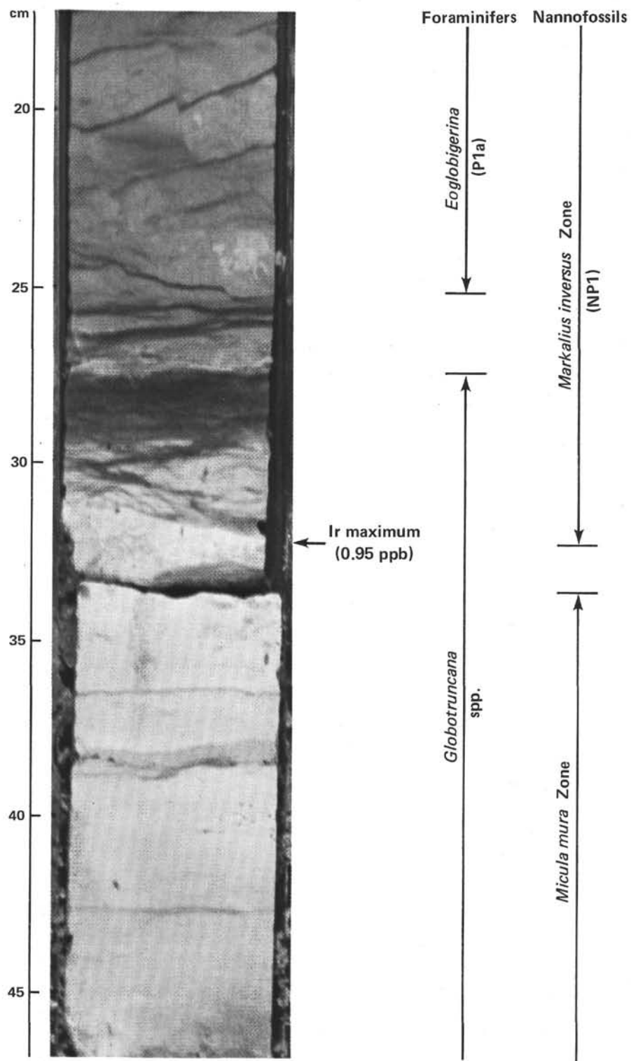
Photograph of Cretaceous/Tertiary boundary in Section 516F-89-5. Ranges of diagnostic foraminifers and nannofossils are shown, based on reports by Pujol, and Weiss (this volume) and site chapter, Site 516 (this volume).
