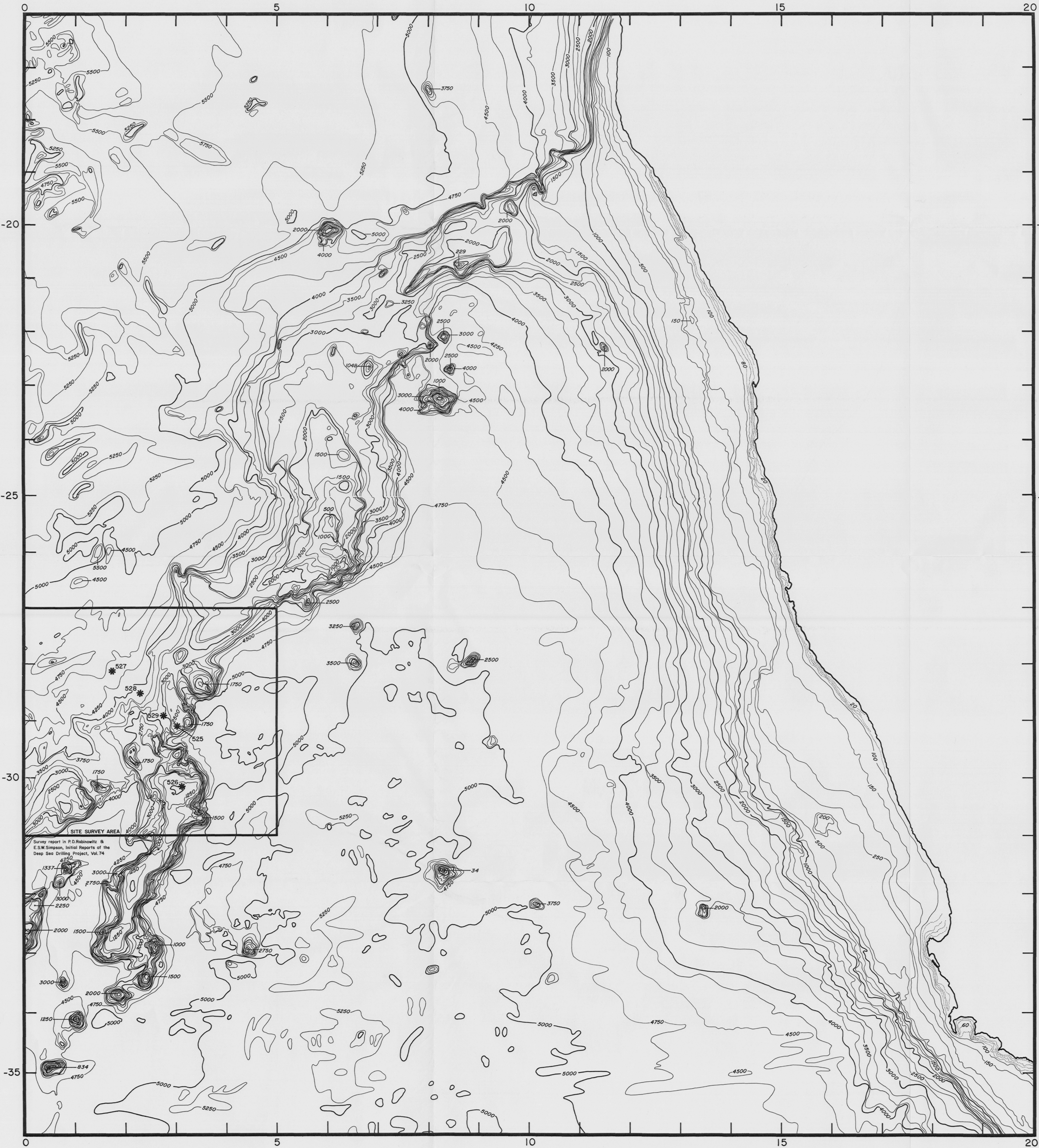
Volume 74: Chapter 30: Figure 4. Bathymetry of the southwestern African margin.
