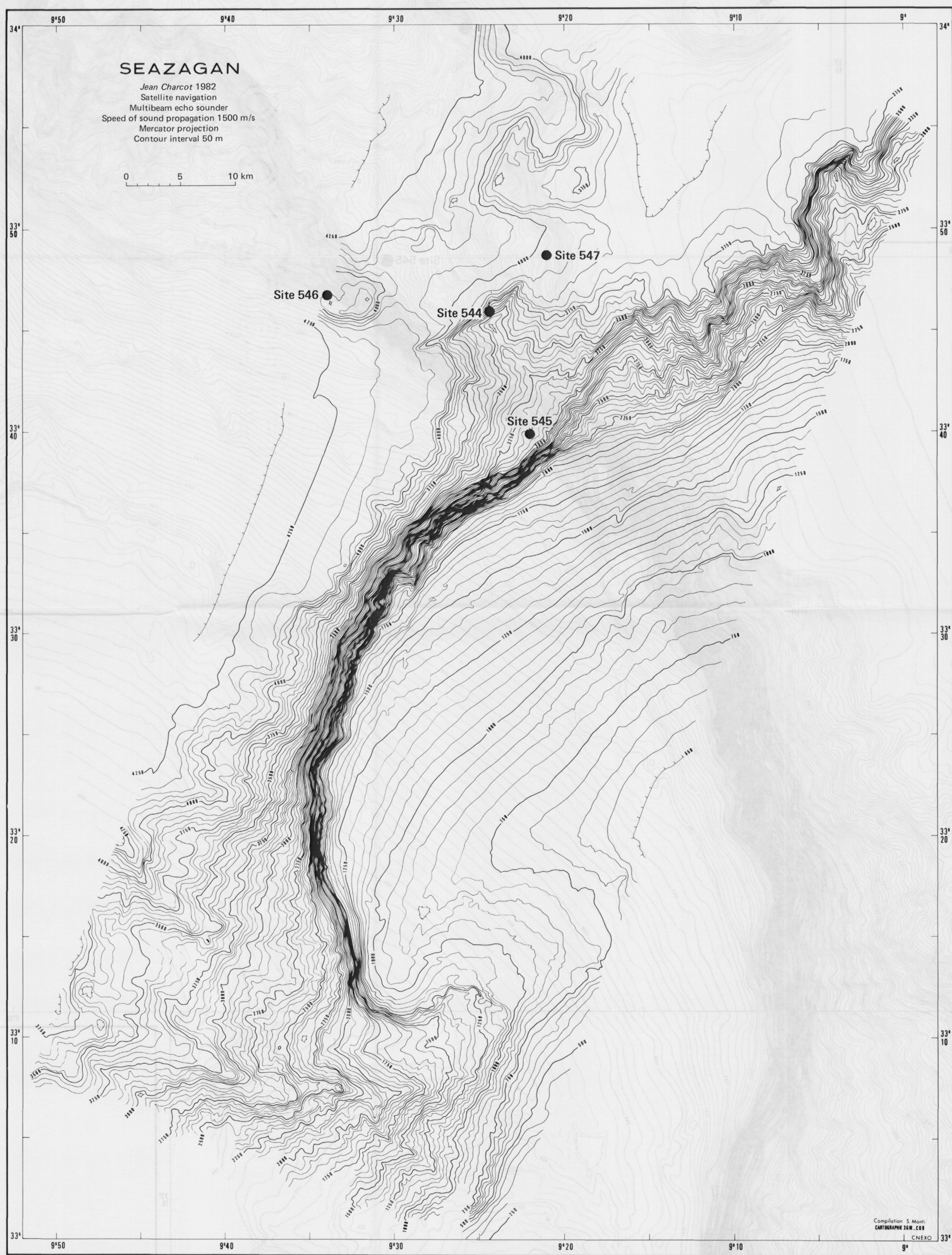
Volume 79: Chapter 6: Figure 4. Seabeam-derived map of the El Jadida Plateau and Escarpment, Scale 1:100,000.
