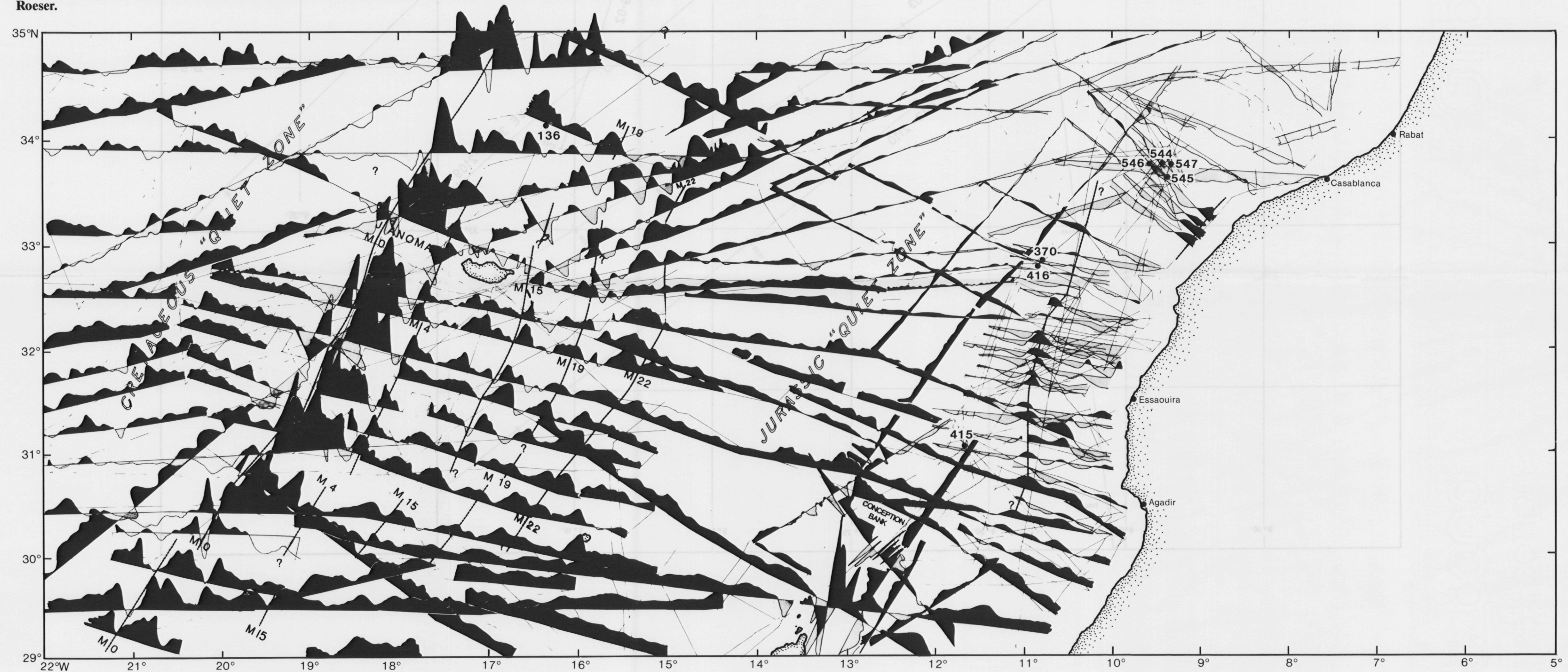
Volume 79: Chapter 38: Figure 3. Magnetic profiles along ships' tracks across the seafloor seaward of the Moroccan continental margin, with correlation of the magnetic anomalies of the M-sequence and of Anomaly S-1 (unlabelled correlation line east of Jurassic "Quiet Zone"). Map prepared by P. D. Rabinowitz, D. E. Hayes, and H. A. Roeser.
