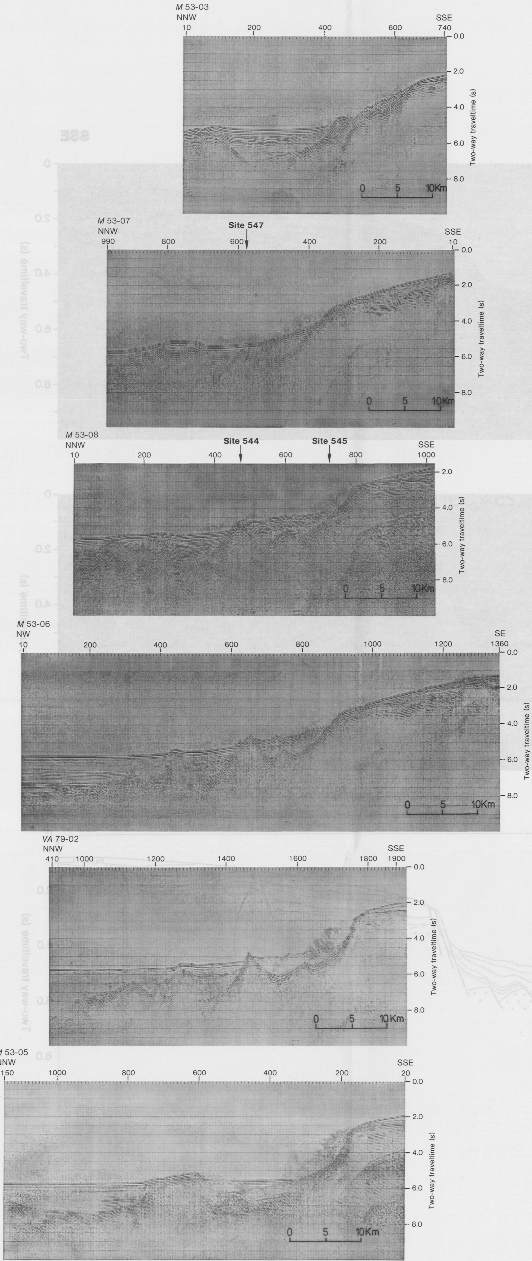
Volume 79: Chapter 38: Figure 6. Multichannel seismic lines from the area of DSDP Leg 79 seaward of the Mazagan Plateau off Central Morocco. Location of lines shown in Figure 5.
