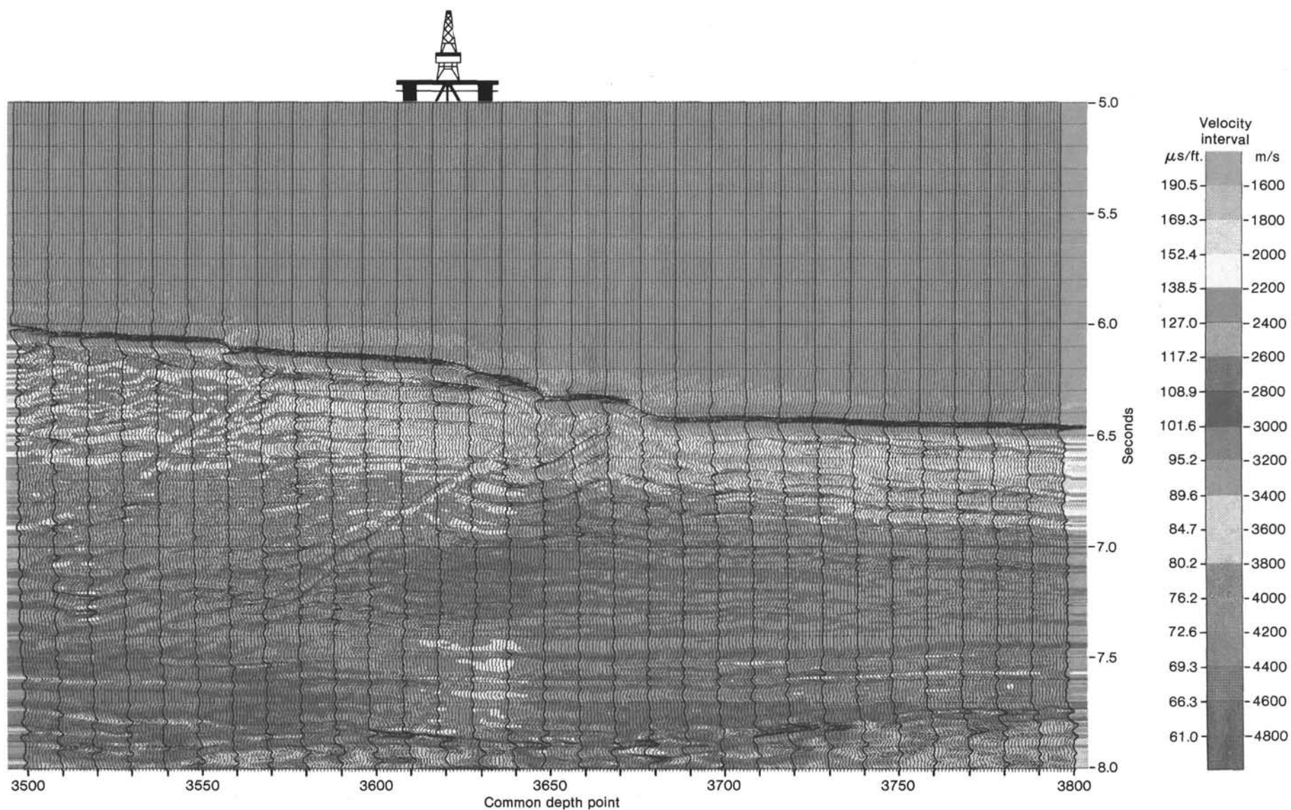
Velocity structure derived from the seismic Profile N55-3-1. Velocities are color coded at every 200 m/s. The rig mark indicates the location of Hole 583F. From Aoki et al., this volume.
