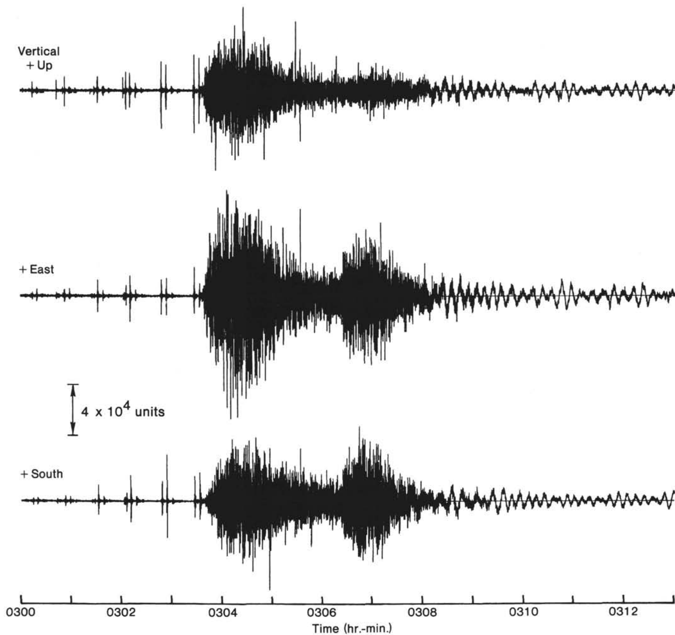
The 26 May 1983 Japan earthquake recorded (unfiltered) by the OSS IV geophones. The spiky arrivals before the earthquake are SUS charge signals.
