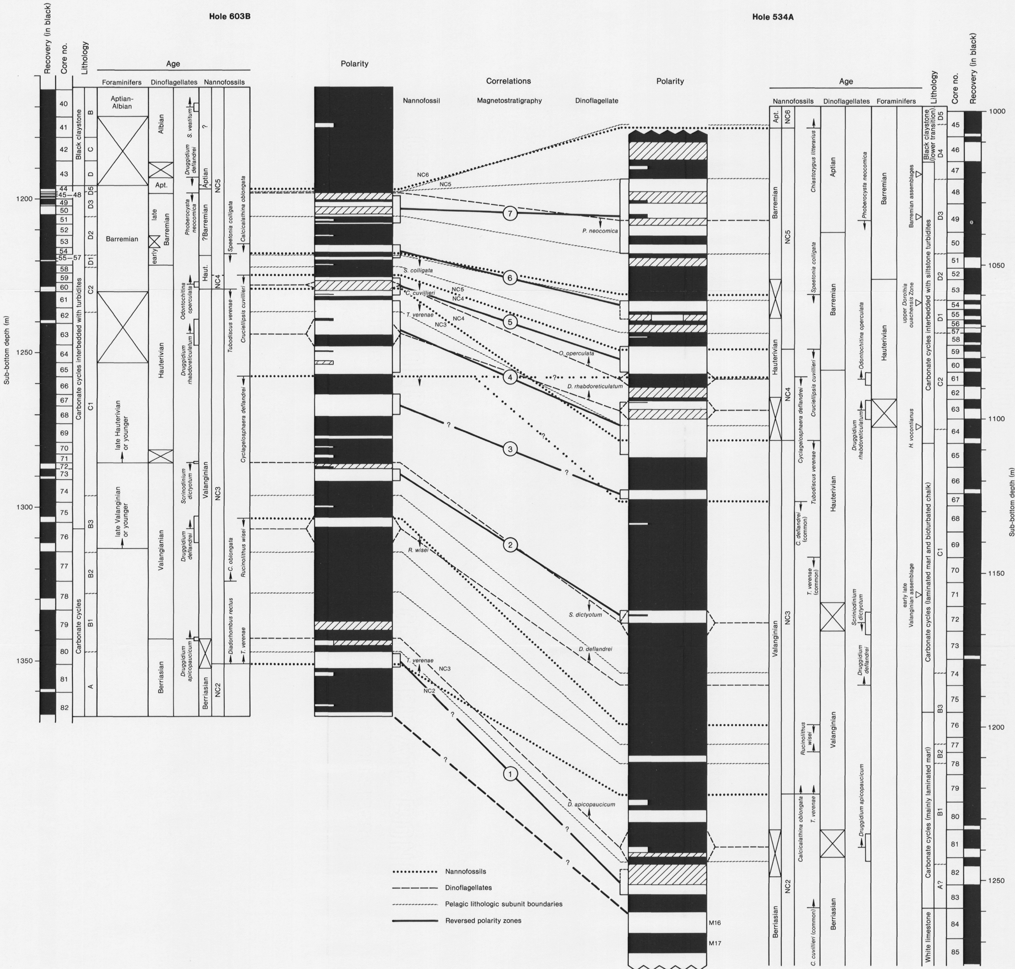
Volume 93: Chapter 31: Figure 9. Early Cretaceous polarity columns for Sites 534 and 603 plotted on a pelagic-sediment stratigraphic scale (all turbidites have been removed from the sections). Possible correlations of major reversed-polarity zones are shown as numbered heavy lines.
