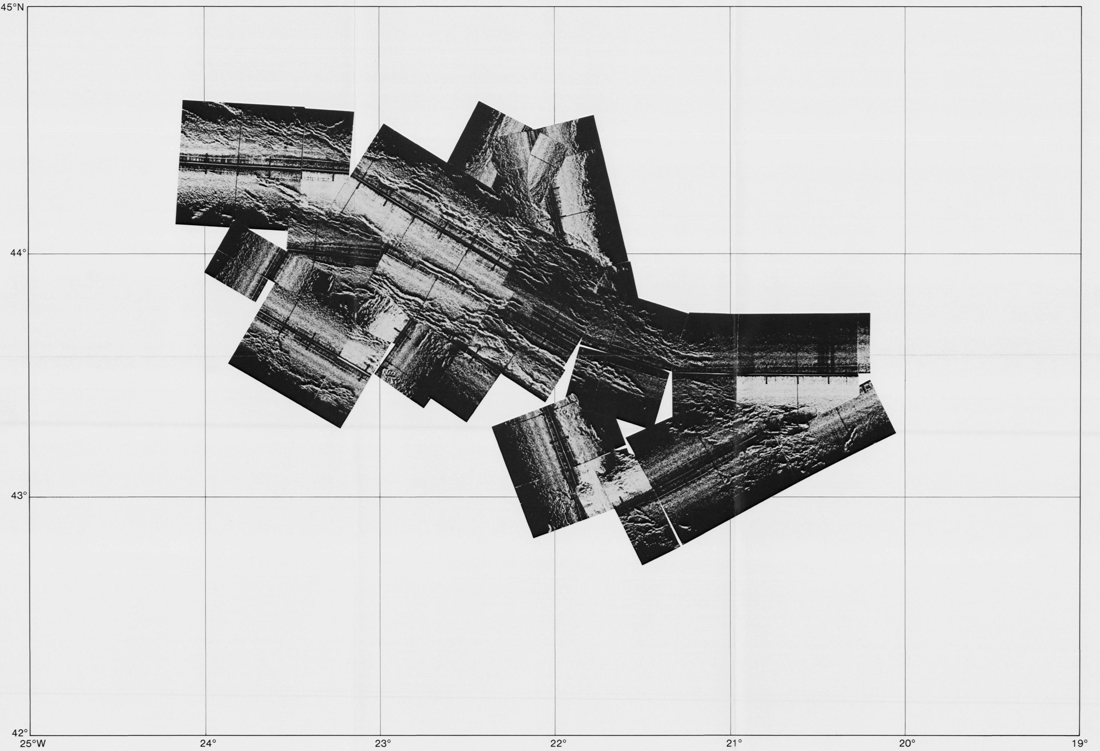
Volume 94: Chapter 49: Figure 3. GLORIA sonograph mosaic of the King's Trough complex. For full interpretation see Kidd et al. (1982). Compare with (overlay) Figure 4 and note the sharp linear (bright) echoes that represent inward-facing fault scarps. See Figure 10 for location of the dredge haul that sampled outcrops on these fault scarps.
