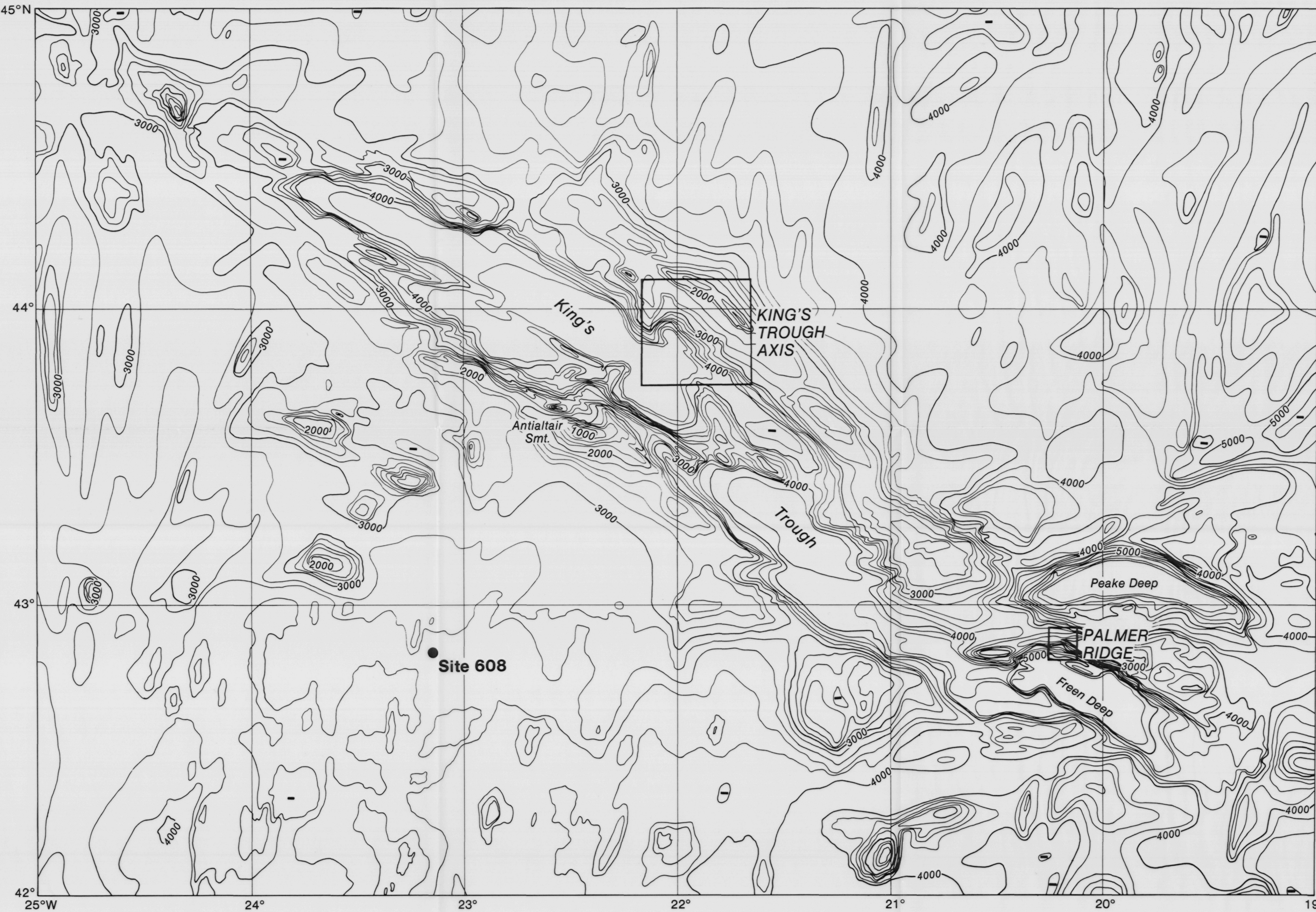
Volume 94: Chapter 49: Figure 4. Bathymetry of King's Trough in corrected meters showing the locations of detailed dredge and rock core sampling at King's Trough Axis and Palmer Ridge and of drilling at Site 608. A basic map constructed by Searle and Whitmarsh (1978) was modified to match sonograph coverage for Kidd et al. (1982). This version includes new sounding data collected for Kidd et al. (1983), compiled and redrafted by Peter Hunter at the Institute of Oceanographic Sciences.
