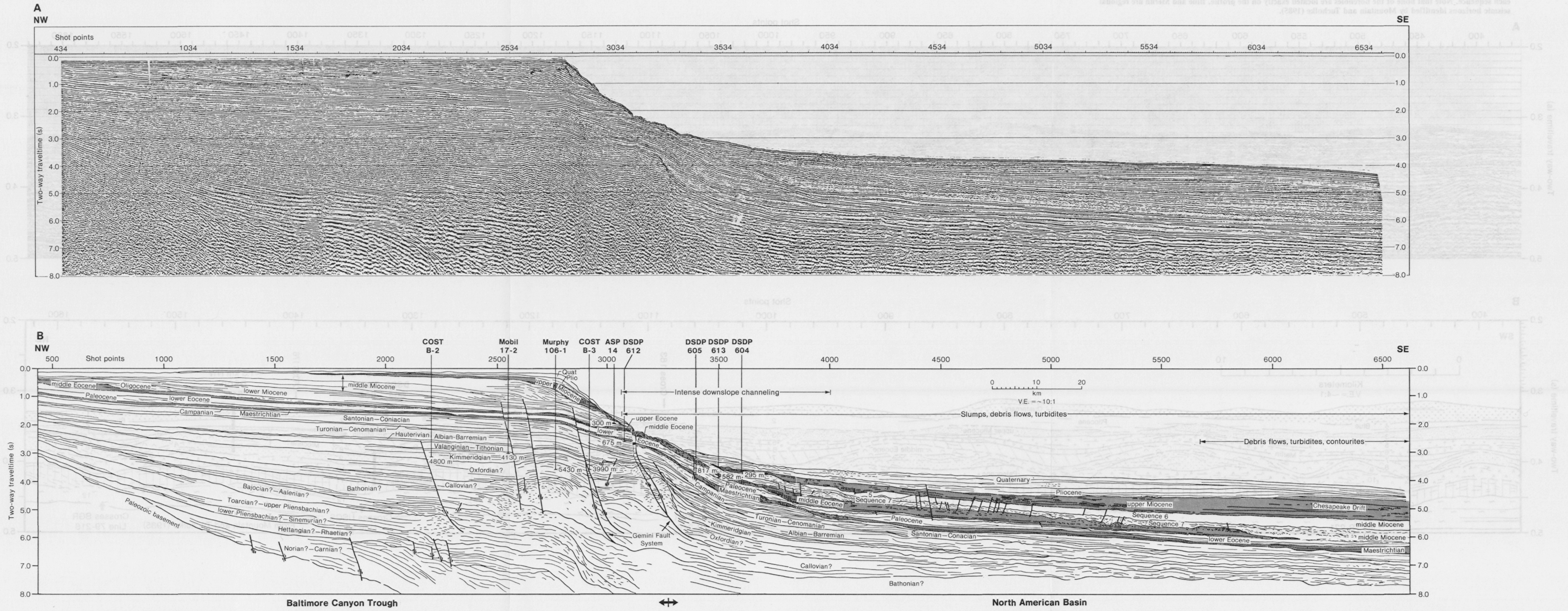
Volume 95: Chapter 32: Figure 20. A. Uninterpreted seismic section, USGS multichannel Profile 25. B. Stratigraphic interpretation of USGS multichannel seismic Profile 25. Shaded sequences are for visual enhancement only. Sequences 7 and 6 can be traced along the Conrad 21 profile to Site 603, where microfossils show that they are of middle Miocene age. Profile Conrad 21 intersects Profile 25 at approximately shot point 6300.
