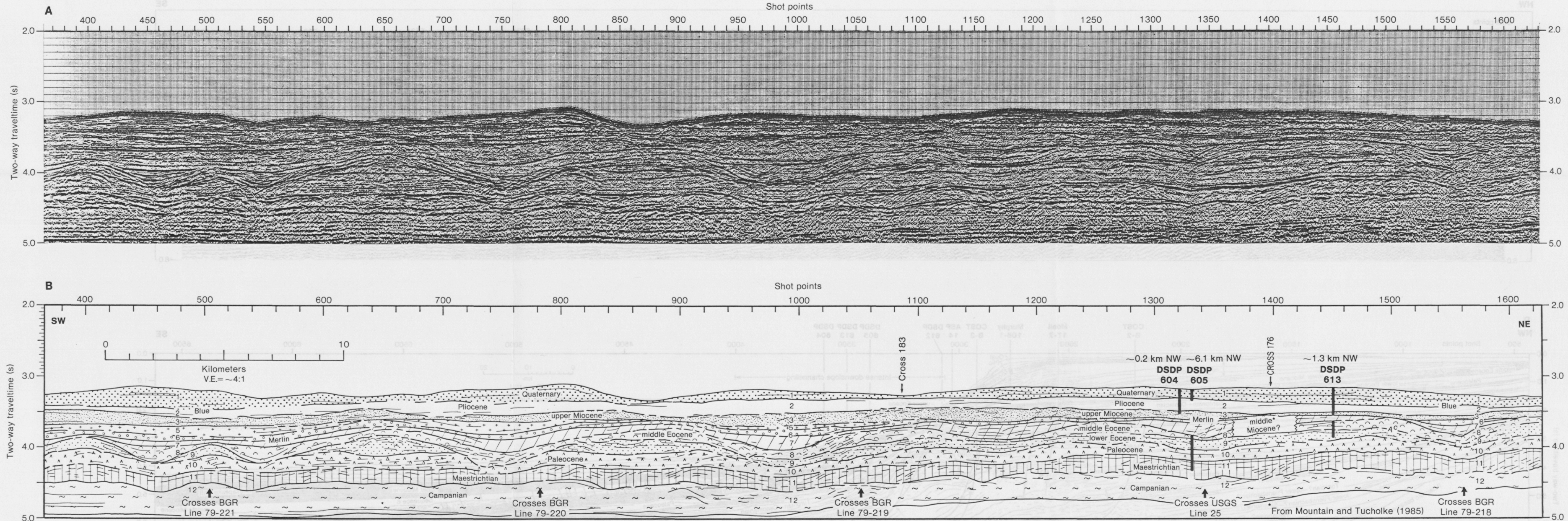
Volume 95: Chapter 32: Figure 24. A. Uninterpreted segment of USGS multichannel seismic Profile 35, a strike section, which intersects Profile 25 along the upper continental rise. B. Stratigraphic interpretation of USGS multichannel seismic Profile 35 showing the series of buried, stacked, erosional channels (modified from Poag, 1985a). Sequences 7 and 6 can be traced to Site 603 where microfossil dating indicates a middle Miocene age for each sequence. Note that none of the boreholes are located exactly on the profile. Blue and Merlin are regional seismic horizons identified by Mountain and Tucholke (1985).
